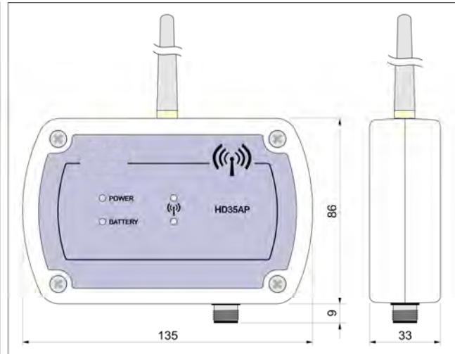
HD35APS
